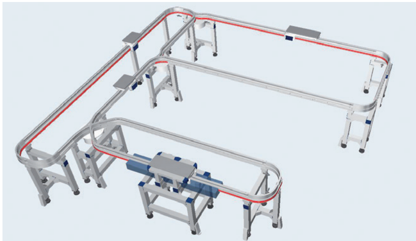
Simple montrac® system with TracControl 1 control
